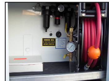
Remote engine controls in right front compartment.
