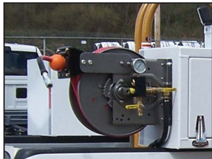
Hose reels available in right front compartment or installed on rear of right side mid-body compartment. 1/2" X 50' heavy duty reel with hose end guard and optional airing station shown.
